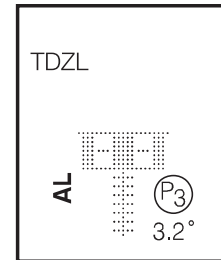
TDZL, PAPI with Lighting Diagram
